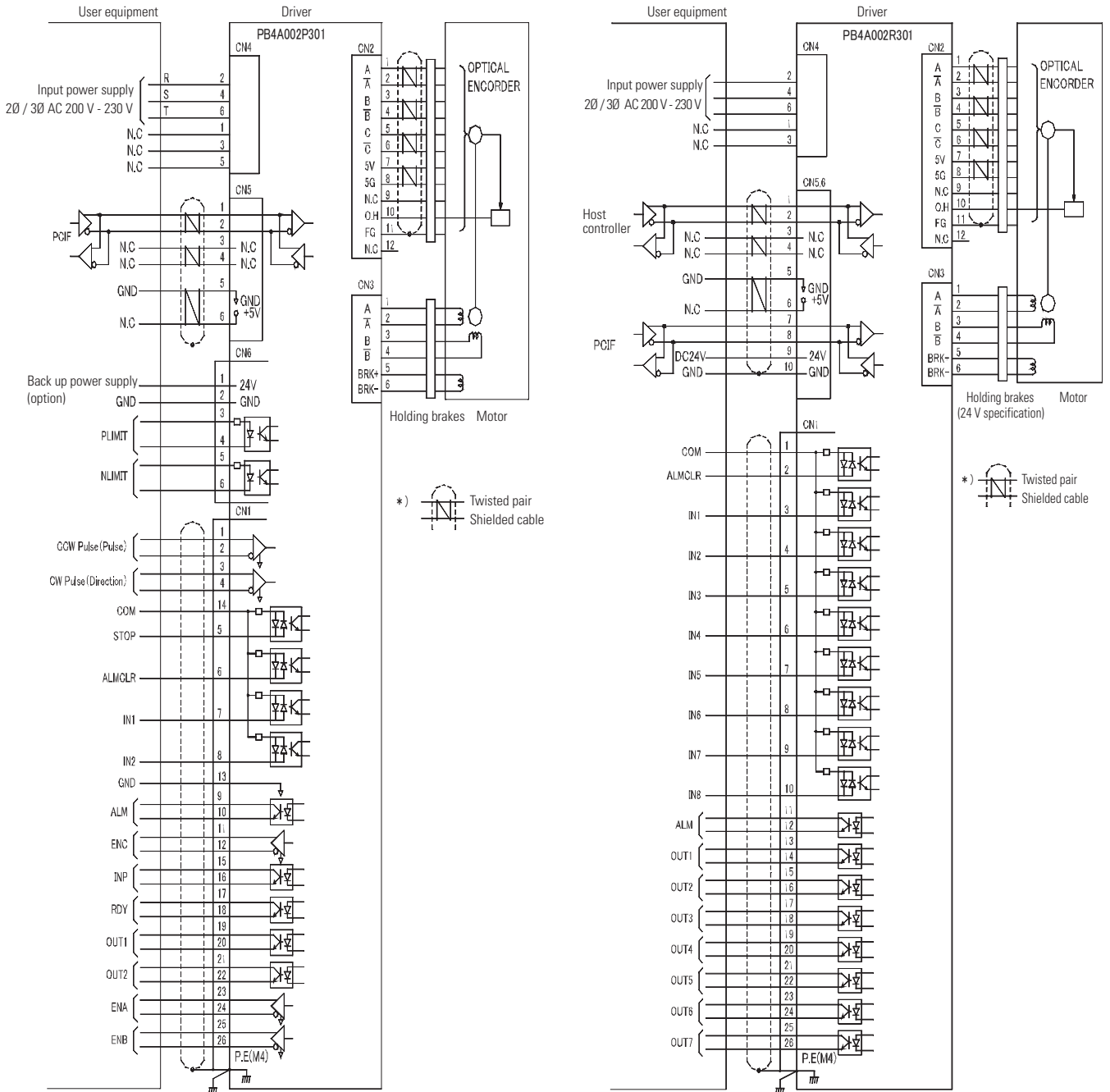
Fig. 2 External wiring diagram (for AC 200 V input)
