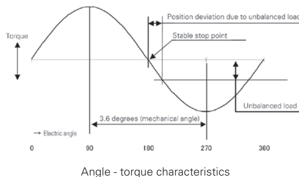
Fig. 5: Outline of position error by the unbalanced load
